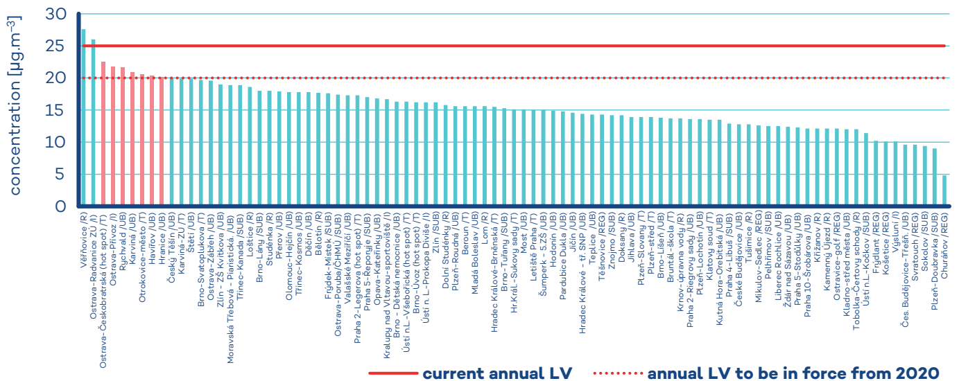
Fig. 2 Annual average concentrations of PM 2.5 in 2019 with LV to be in force from 2020
