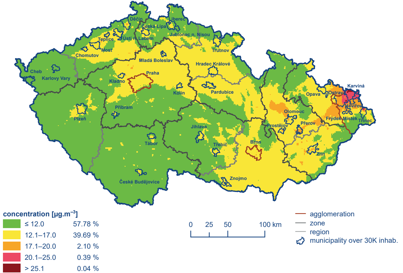
Fig. 1 Field of annual average concentration of PM 2.5 in 2019 indicating limit value valid from 2020
