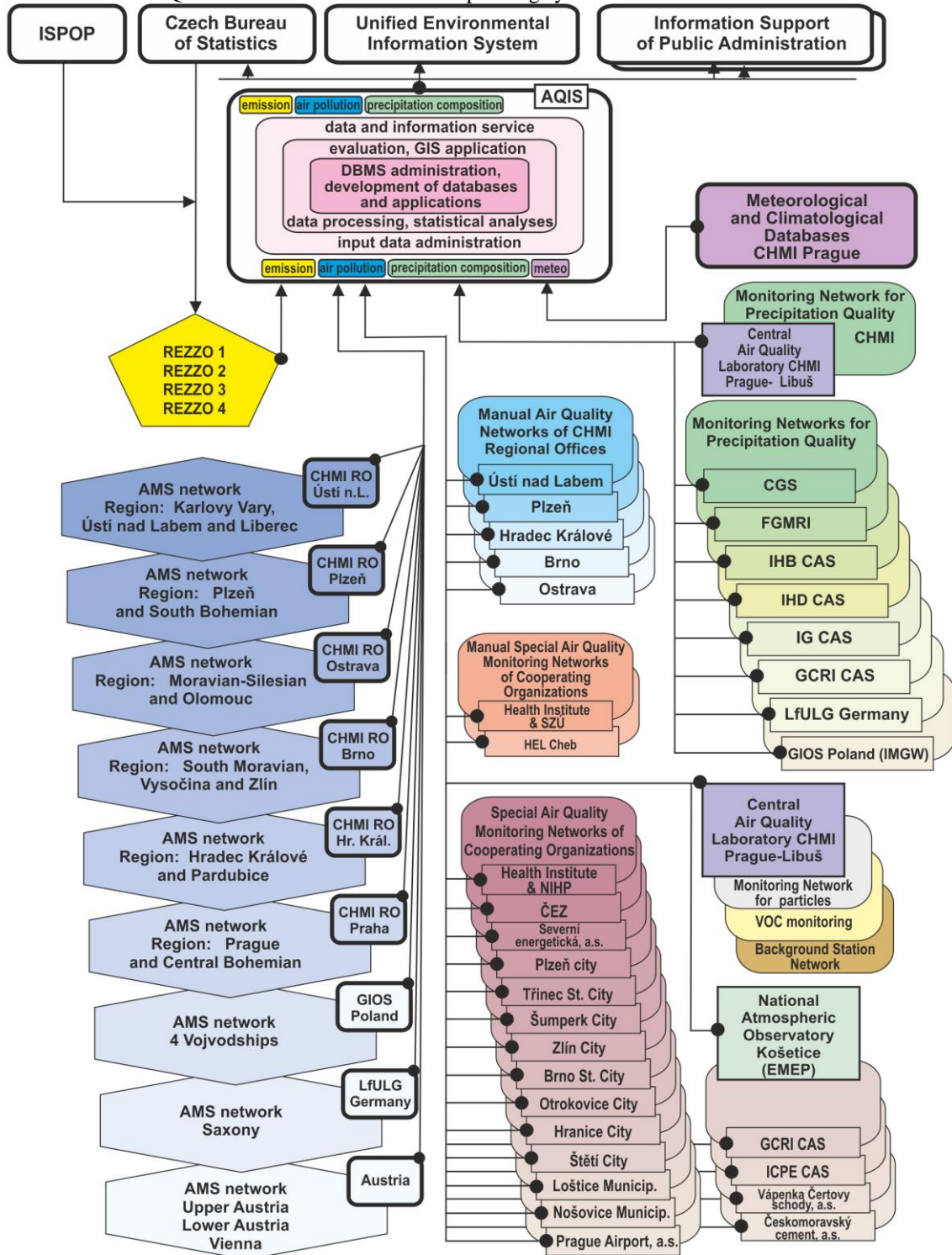
Fig. 1 Scheme of the AQIS links to data sources and cooperating systems in 2018
